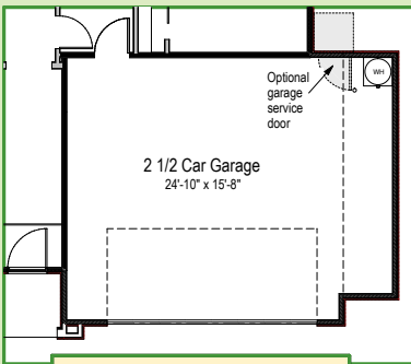
2 1/2 CAR OPTION
